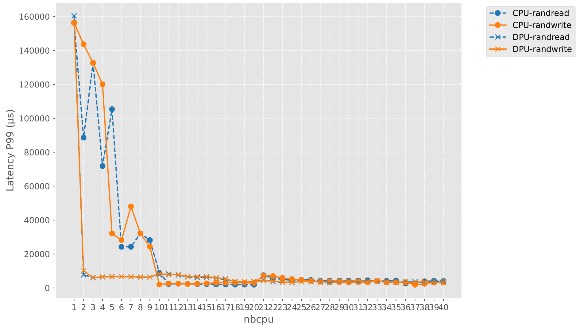
Latency P99 vs nbcpu (CPU vs DPU)
